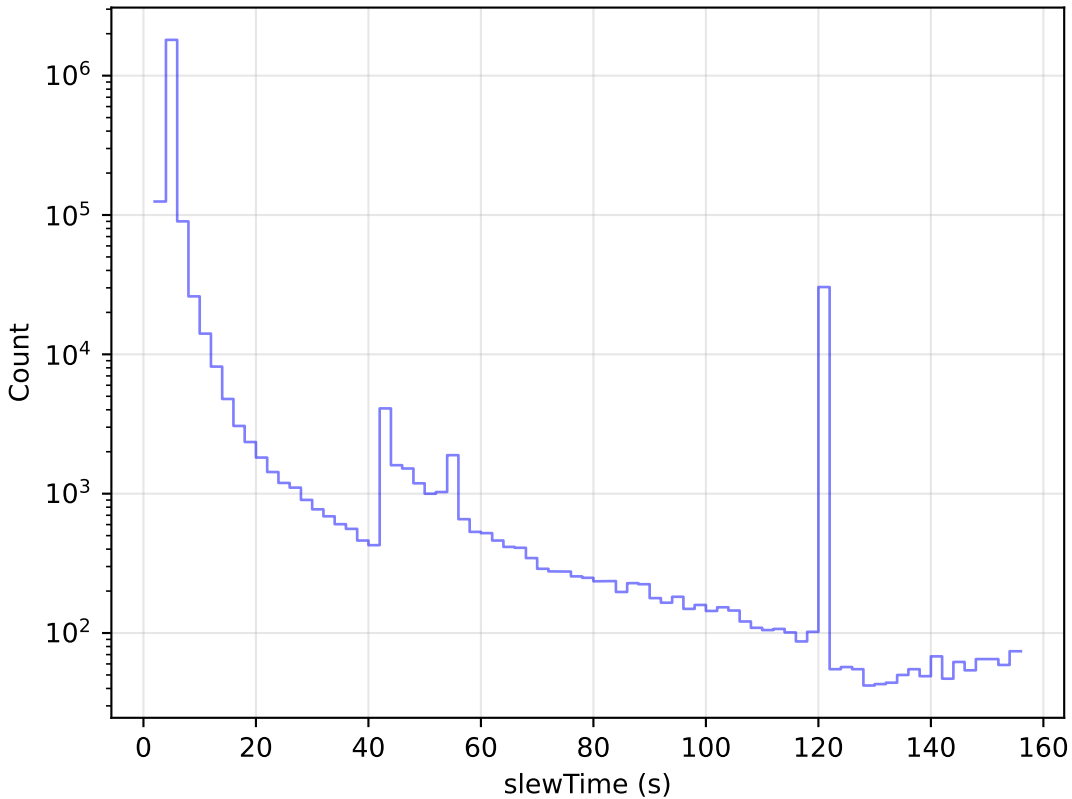
ddf_acor_sf20_lsf0_lsr0_v3.4_10yrs All visits: Slew Time Histogram
