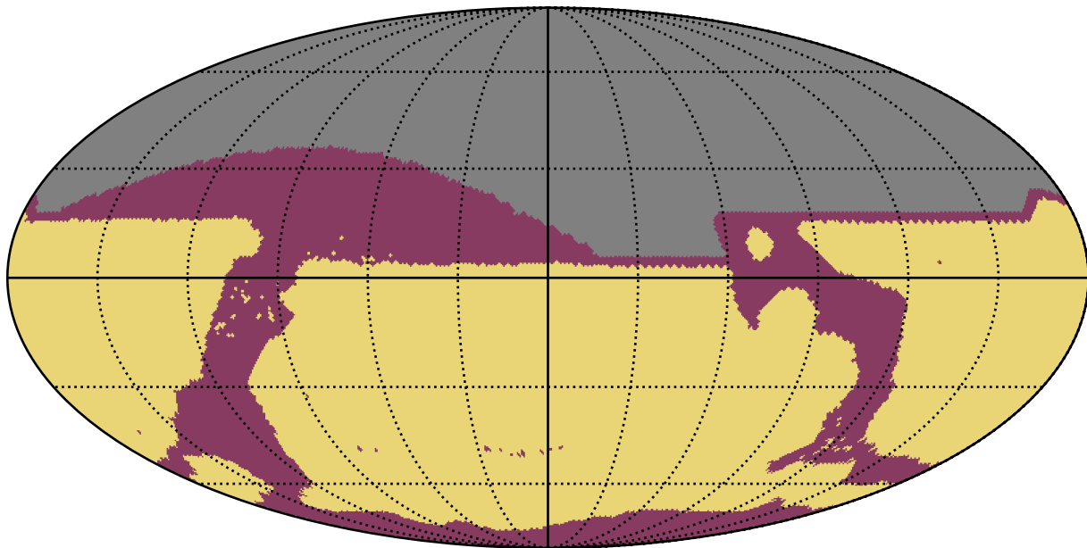
ddf_acor_sf20_lsf0_lsr0_v3.4_10yrs All sky: RapidRevisits
