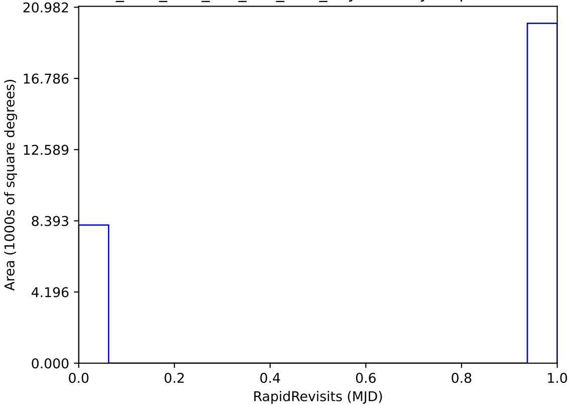
ddf_acor_sf20_lsf0_lsr0_v3.4_10yrs All sky: RapidRevisits
