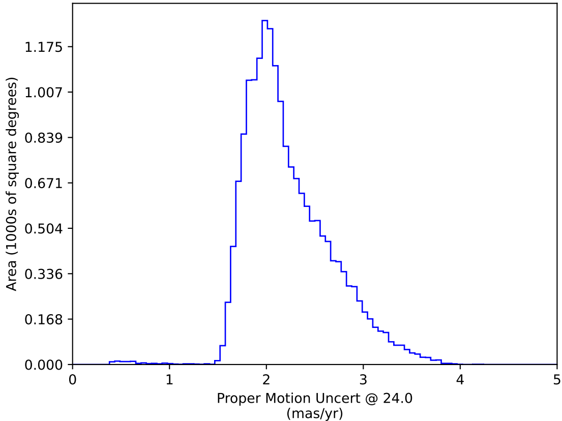
ddf_acor_sf20_lsf0_lsr0_v3.4_10yrs WFD: Proper Motion Uncert @ 24.0
