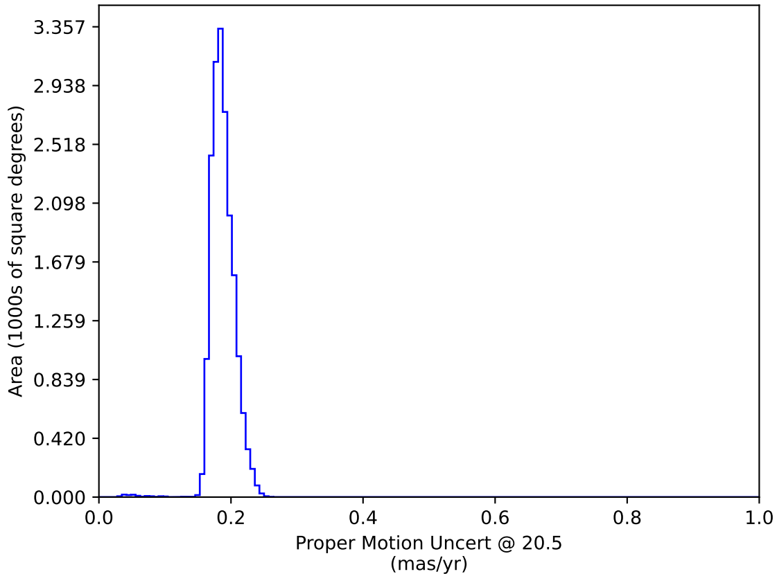
ddf_acor_sf20_lsf0_lsr0_v3.4_10yrs WFD: Proper Motion Uncert @ 20.5
