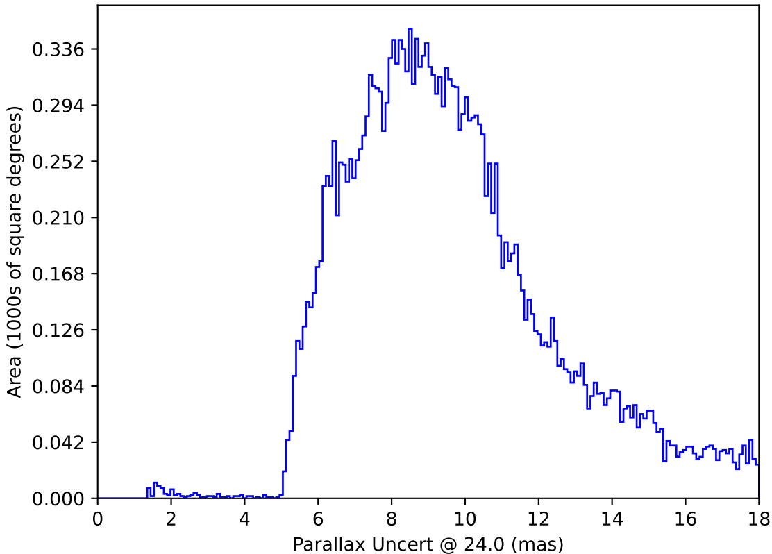
ddf_acor_sf20_lsf0_lsr0_v3.4_10yrs All sky: Parallax Uncert @ 24.0
