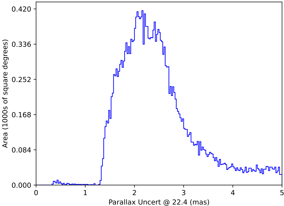
ddf_acor_sf20_lsf0_lsr0_v3.4_10yrs All sky: Parallax Uncert @ 22.4
