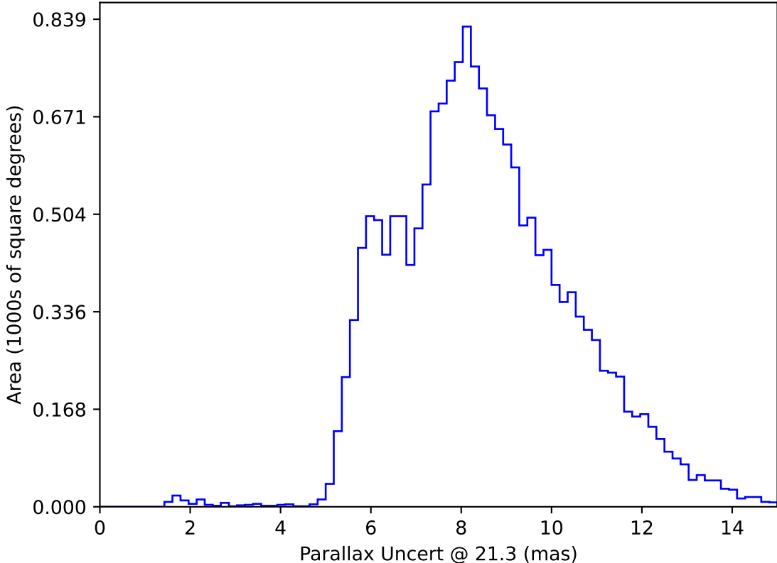
ddf_acor_sf20_lsf0_lsr0_v3.4_10yrs WFD y band only: Parallax Uncert @ 21.3
