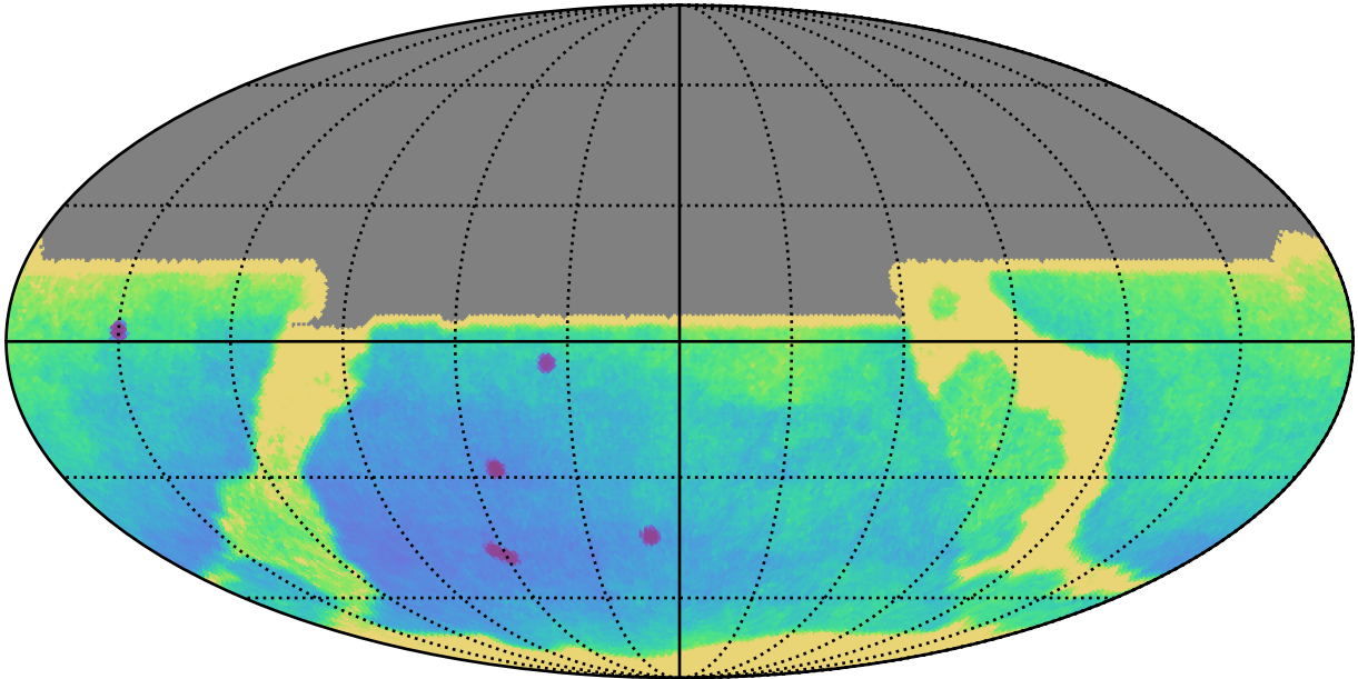
ddf_acor_sf20_lsf0_lsr0_v3.4_10yrs All sky y band only: Parallax Uncert @ 21.3
