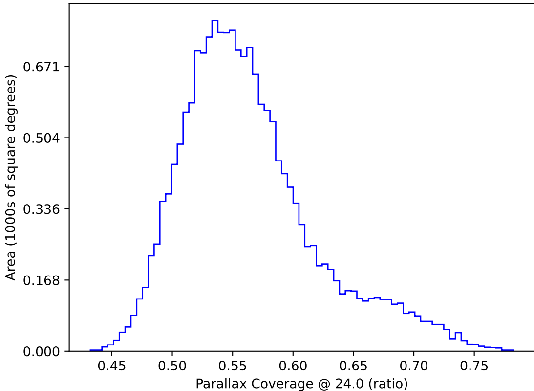
ddf_acor_sf20_ls0_lsr0_v3.4_10yrs WFD: Parallax Coverage @ 24.0
