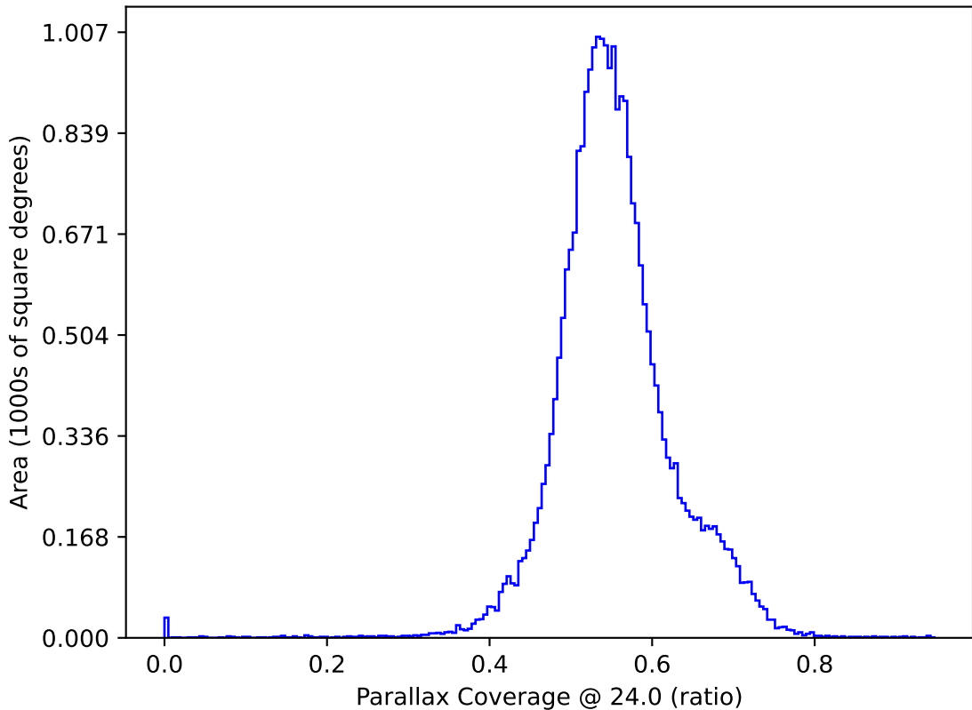
ddf_acor_sf20_lsf0_lsr0_v3.4_10yrs All sky: Parallax Coverage @ 24.0
