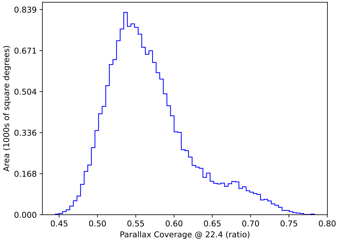
ddf_acor_sf20_lsf0_lsr0_v3.4_10yrs WFD: Parallax Coverage @ 22.4
