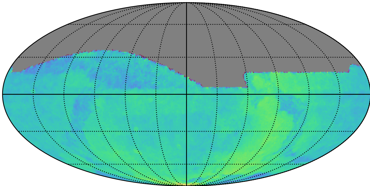
ddf_acor_sf20_lsf0_lsr0_v3.4_10yrs All sky: Parallax Coverage @ 22.4
