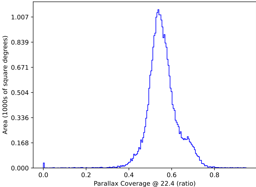
ddf_acor_sf20_lsf0_lsr0_v3.4_10yrs All sky: Parallax Coverage @ 22.4
