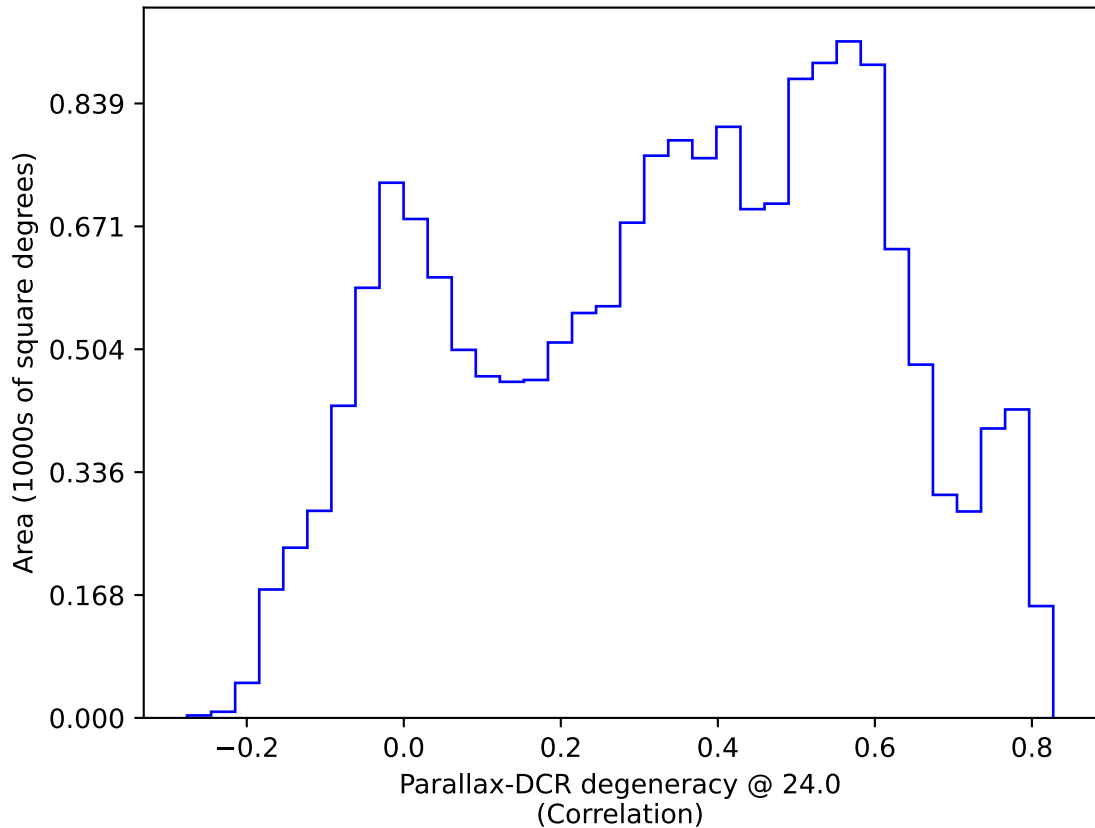
ddf_acor_sf20_lsf0_lsr0_v3.4_10yrs WFD: Parallax-DCR degeneracy @ 24.0
