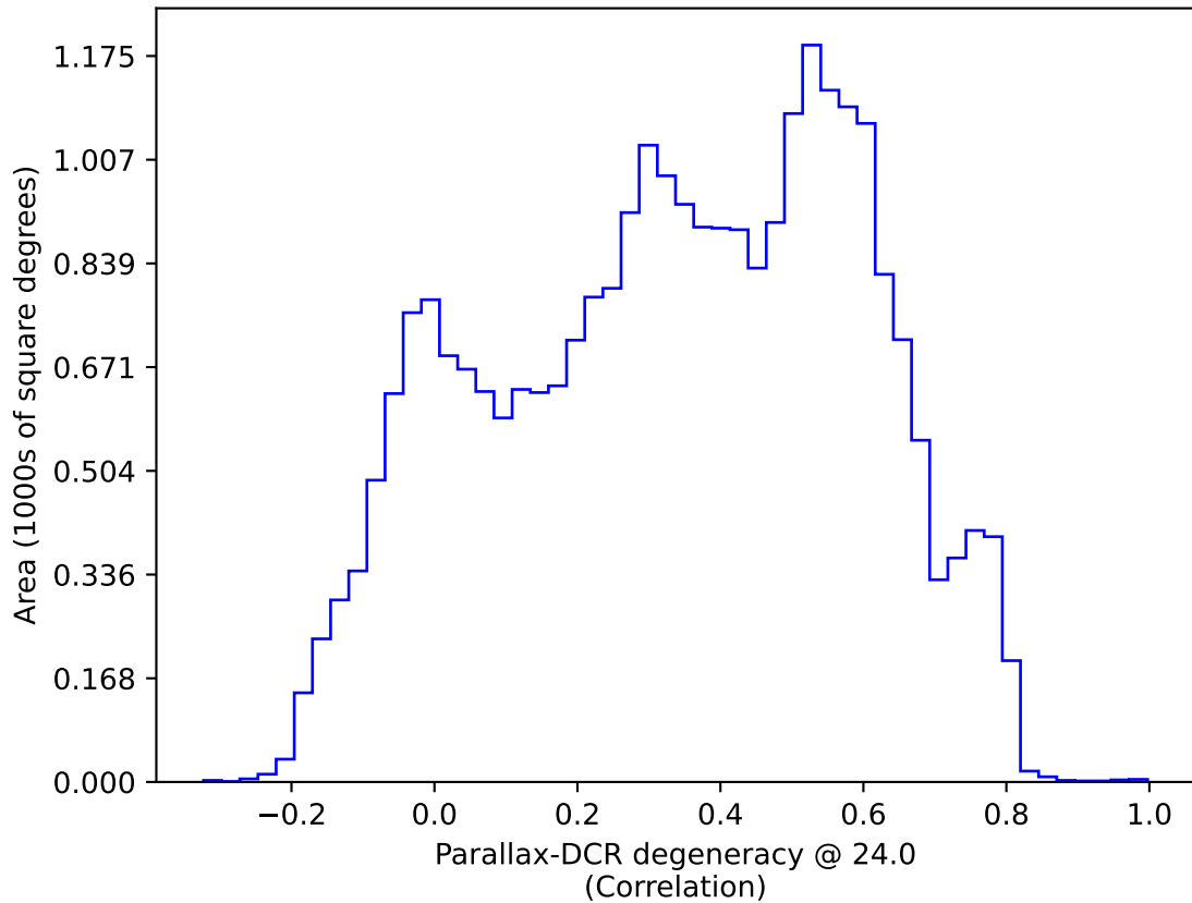
ddf_acor_sf20_ls0_lsr0_v3.4_10yrs All sky: Parallax-DCR degeneracy @ 24.0
