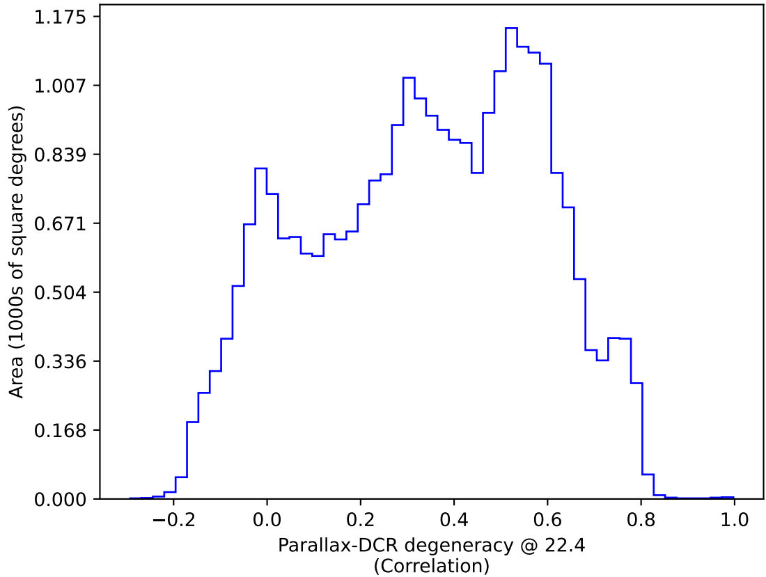
ddf_acor_sf20_ls0_lsr0_v3.4_10yrs All sky: Parallax-DCR degeneracy @ 22.4
