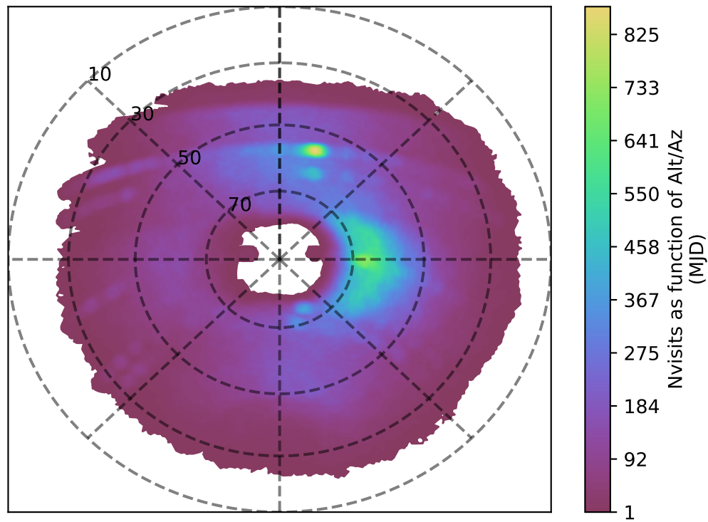
ddf_acor_sf20_lsf0_lsr0_v3.4_10yrs u band: Nvisits as function of Alt/Az
