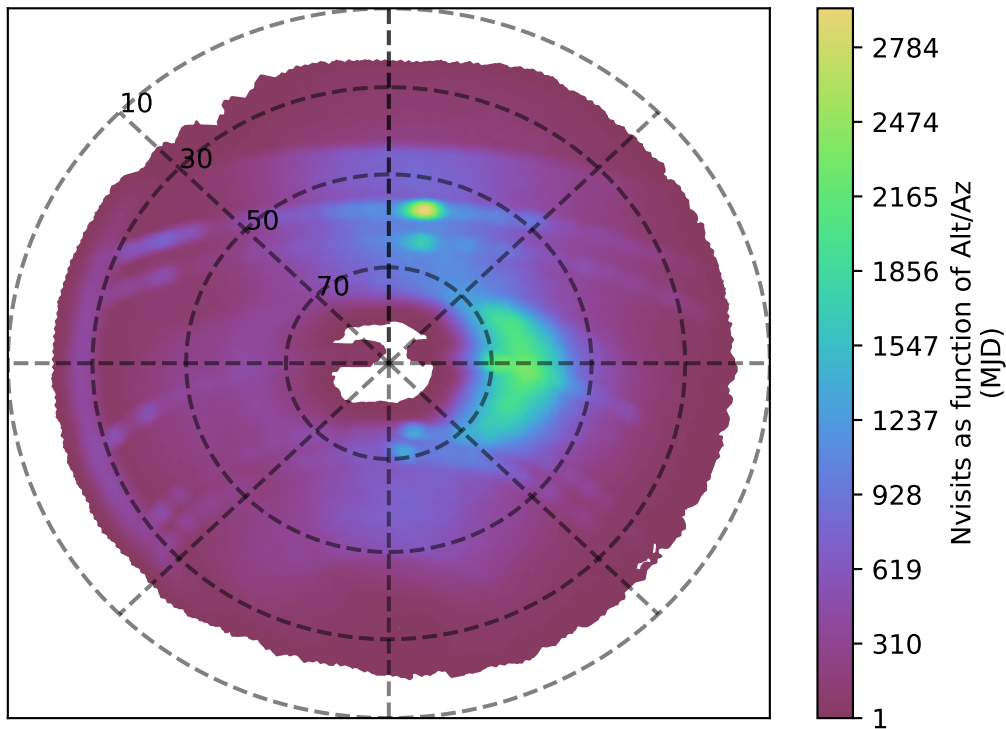
ddf_acor_sf20_lsf0_lsr0_v3.4_10yrs r band: Nvisits as function of Alt/Az
