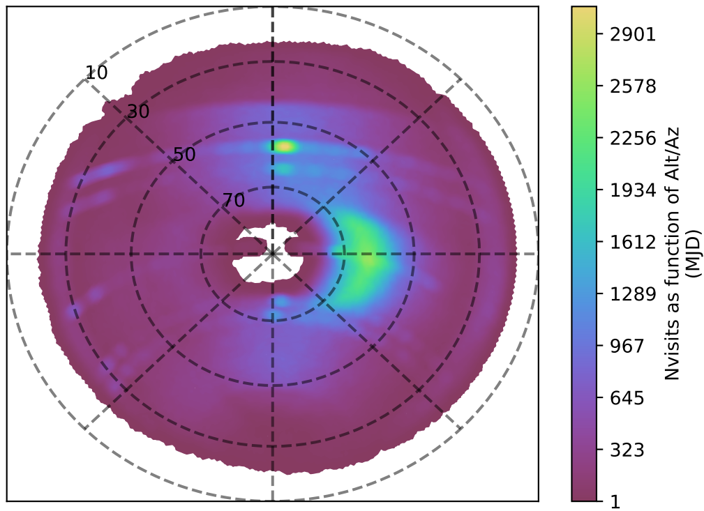
ddf_acor_sf20_lsf0_lsr0_v3.4_10yrs i band: Nvisits as function of Alt/Az
