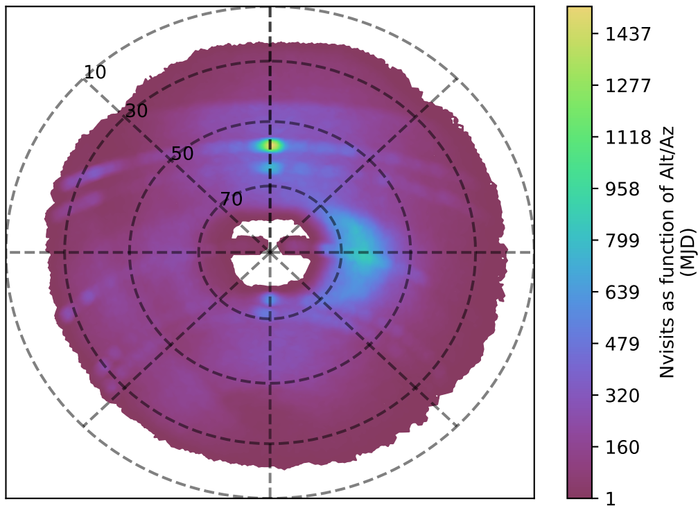
ddf_acor_sf20_lsf0_lsr0_v3.4_10yrs g band: Nvisits as function of Alt/Az
