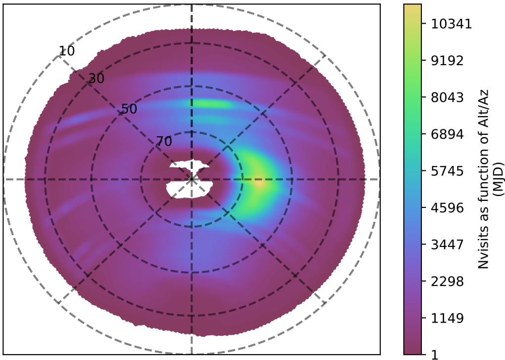
ddf_acor_sf20_lsf0_lsr0_v3.4_10yrs all bands: Nvisits as function of Alt/Az
