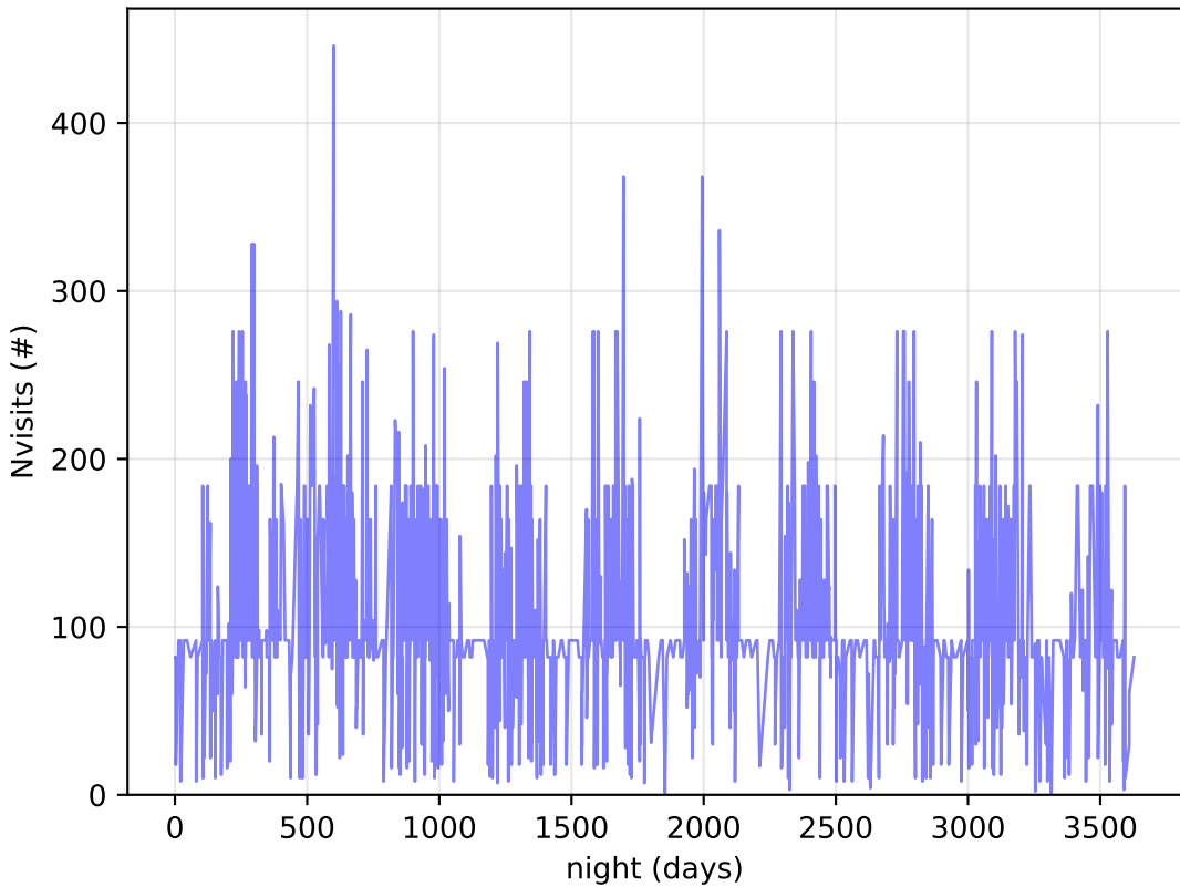
ddf_acor_sf20_lsf0_lsr0_v3.4_10yrs DDF: Nvisits
