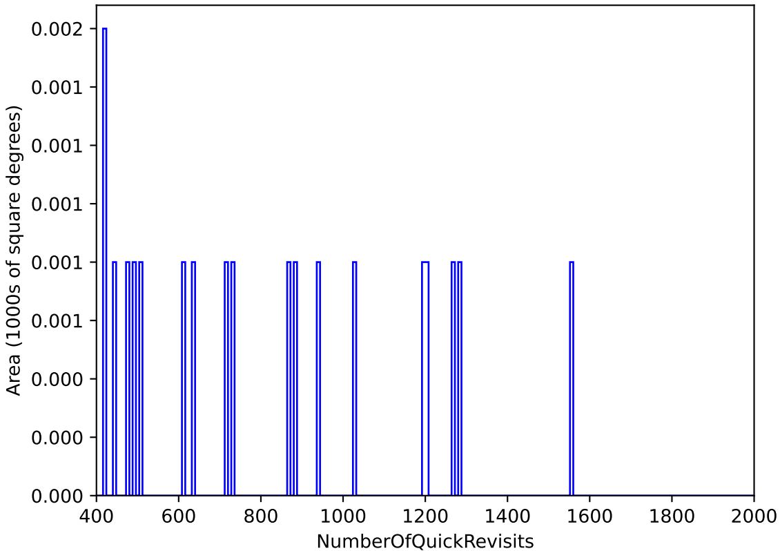
ddf_acor_sf20_lsf0_lsr0_v3.4_10yrs WFD: NumberOfQuickRevisits
