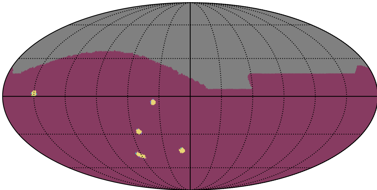
ddf_acor_sf20_lsf0_lsr0_v3.4_10yrs All sky: NumberOfQuickRevisits
