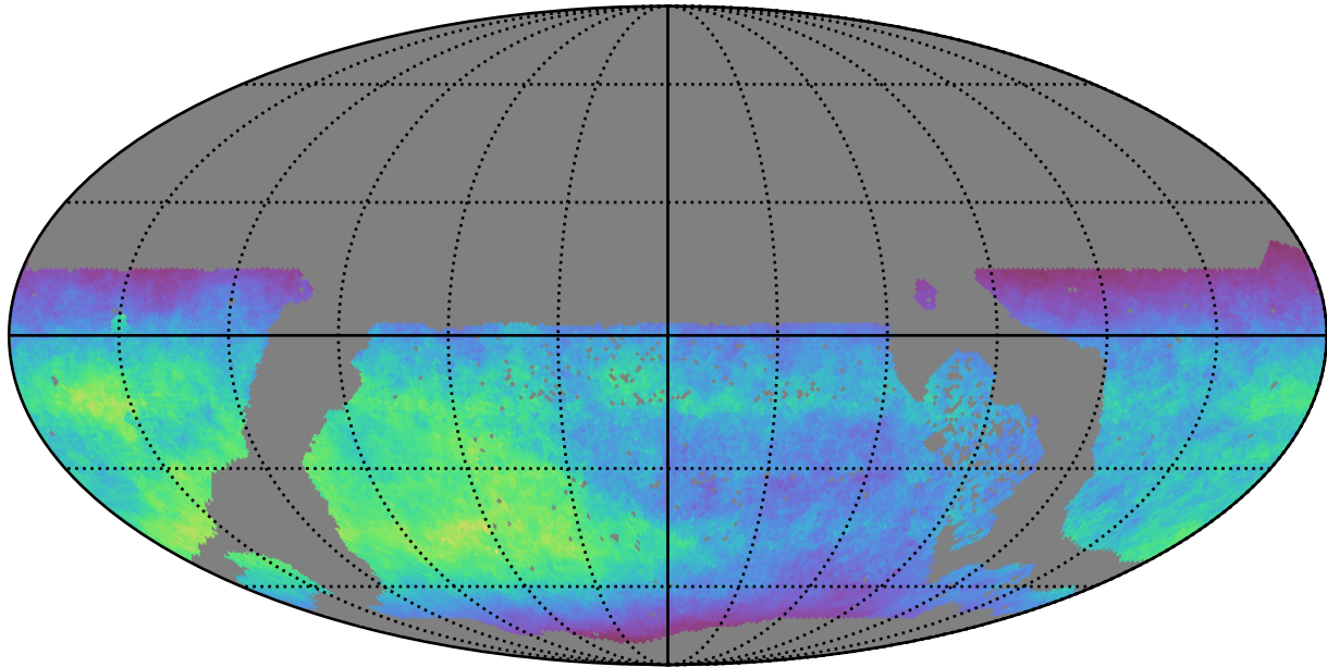
ddf_acor_sf20_lsf0_lsr0_v3.4_10yrs WFD z band: Normalized Teff
