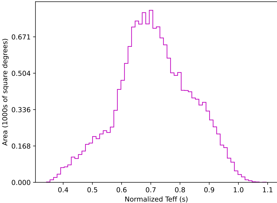
ddf_acor_sf20_lsf0_lsr0_v3.4_10yrs WFD z band: Normalized Teff
