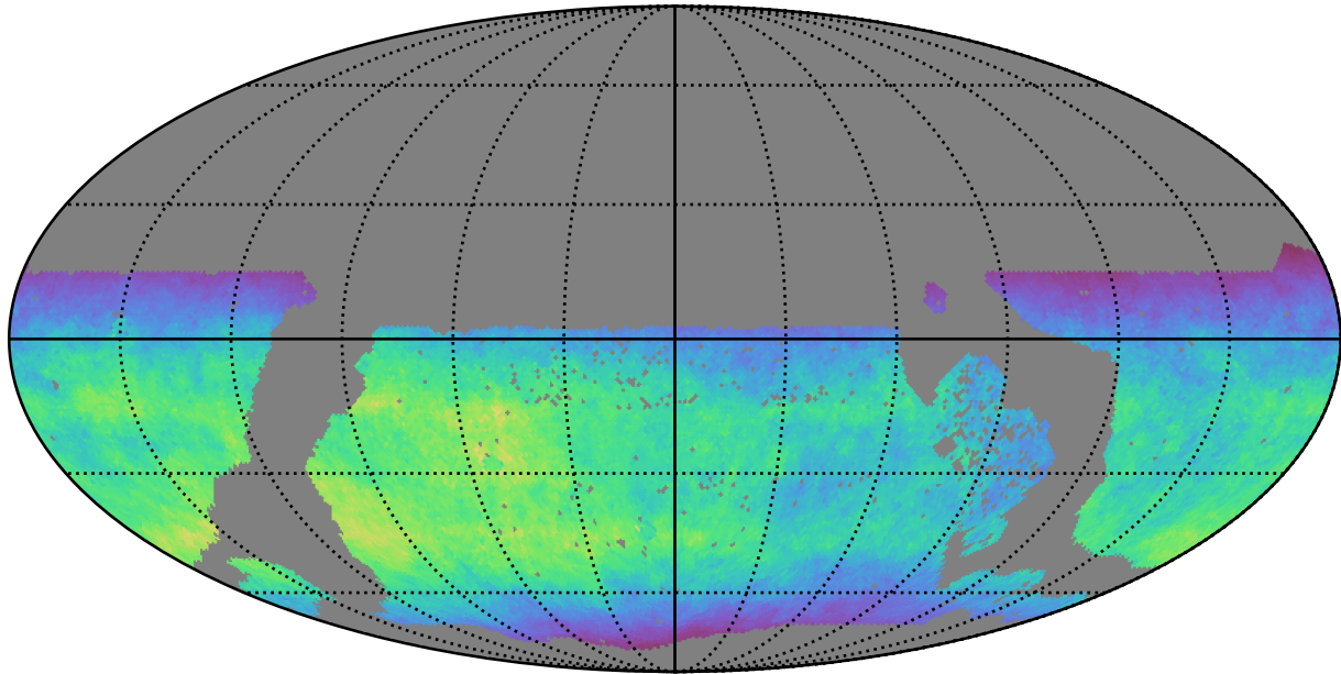
ddf_acor_sf20_lsf0_lsr0_v3.4_10yrs WFD y band: Normalized Teff
