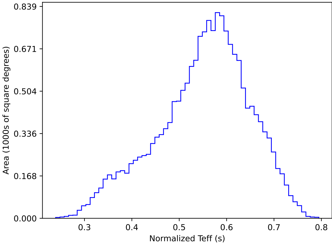
ddf_acor_sf20_lsf0_lsr0_v3.4_10yrs WFD y band: Normalized Teff
