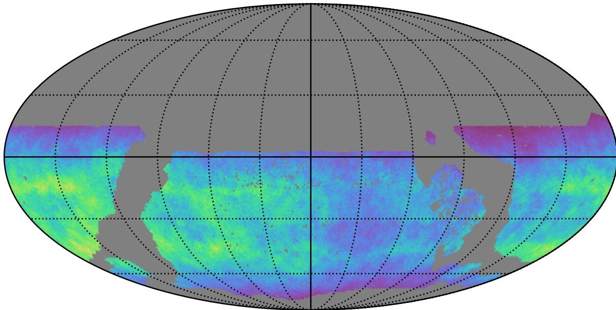
ddf_acor_sf20_lsf0_lsr0_v3.4_10yrs WFD u band: Normalized Teff
