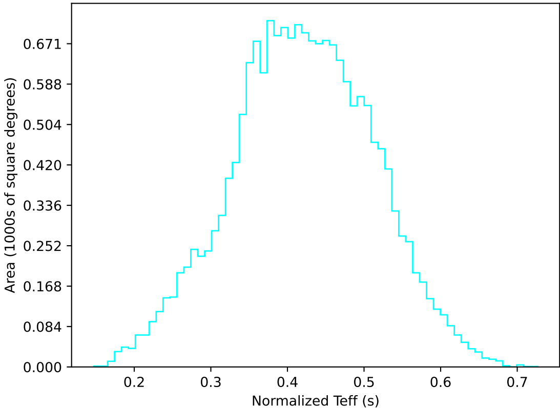
ddf_acor_sf20_lsf0_lsr0_v3.4_10yrs WFD u band: Normalized Teff
