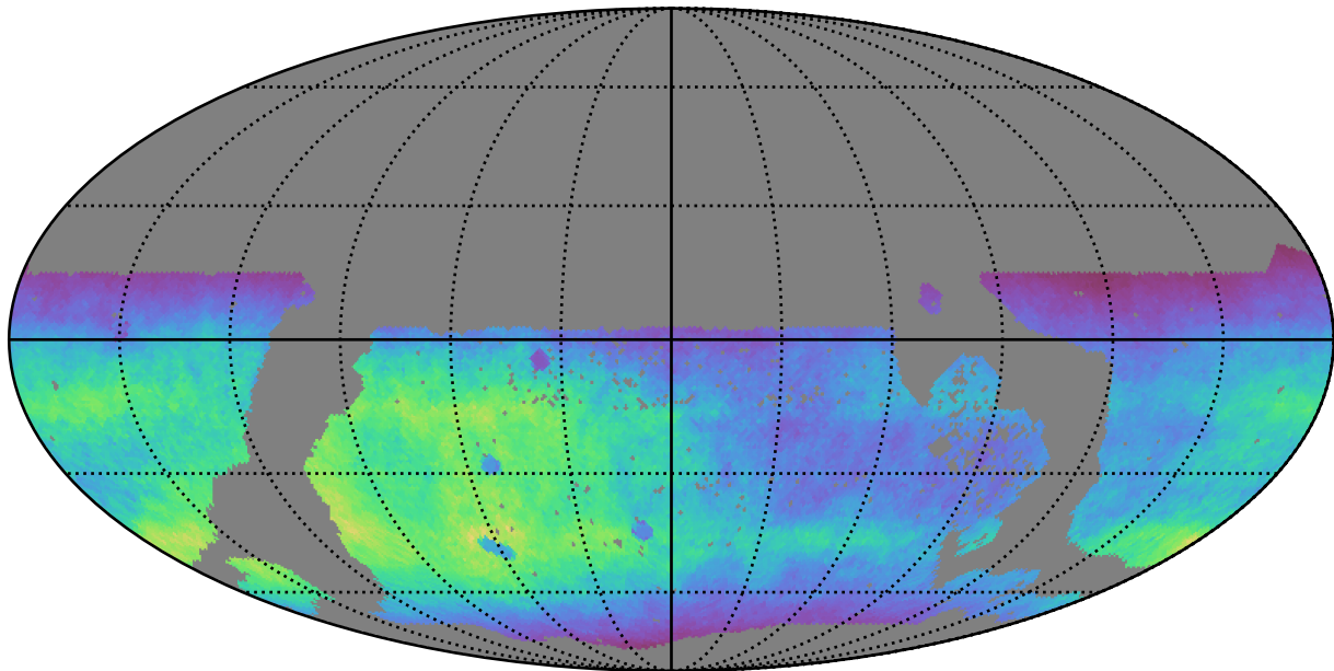
ddf_acor_sf20_lsf0_lsr0_v3.4_10yrs WFD r band: Normalized Teff
