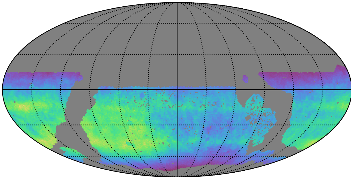
ddf_acor_sf20_lsf0_lsr0_v3.4_10yrs WFD i band: Normalized Teff
