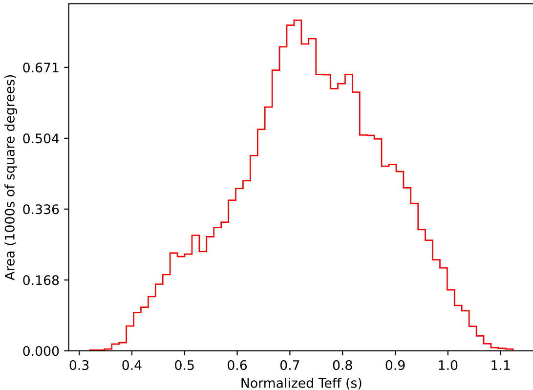
ddf_acor_sf20_lsf0_lsr0_v3.4_10yrs WFD i band: Normalized Teff
