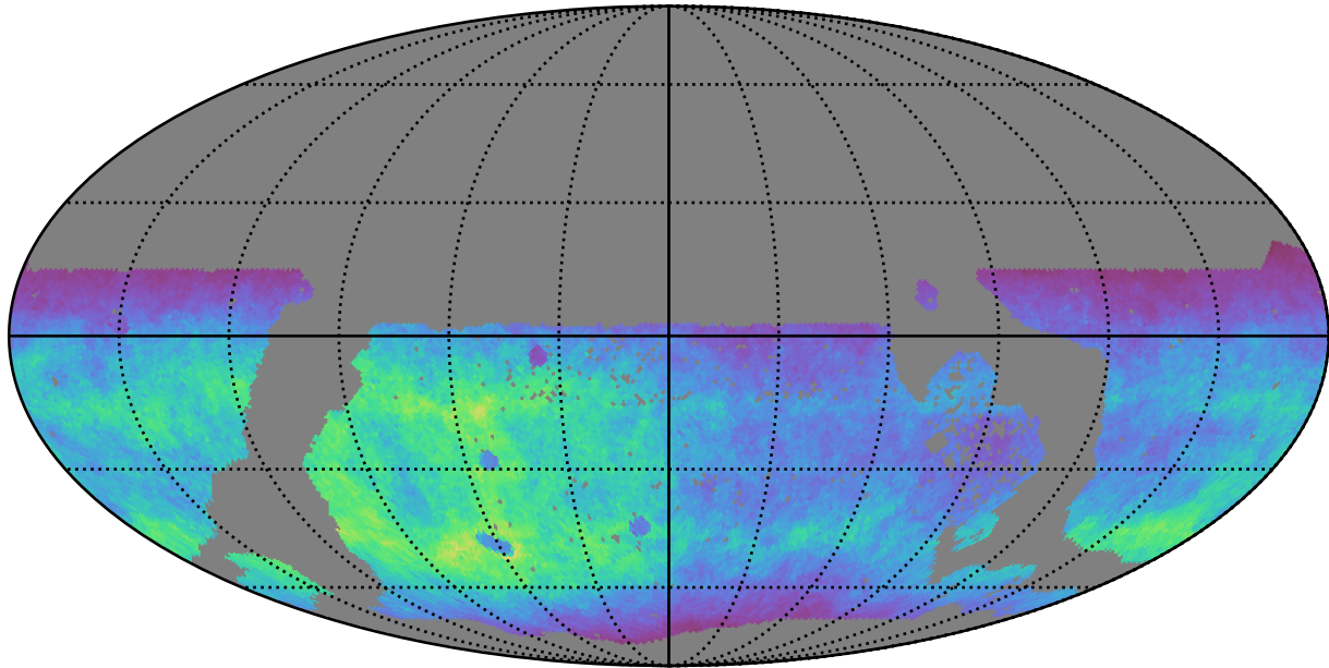
ddf_acor_sf20_lsf0_lsr0_v3.4_10yrs WFD g band: Normalized Teff
