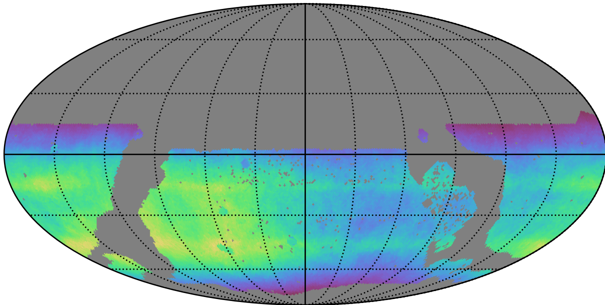
ddf_acor_sf20_lsf0_lsr0_v3.4_10yrs WFD all bands: Normalized Teff
