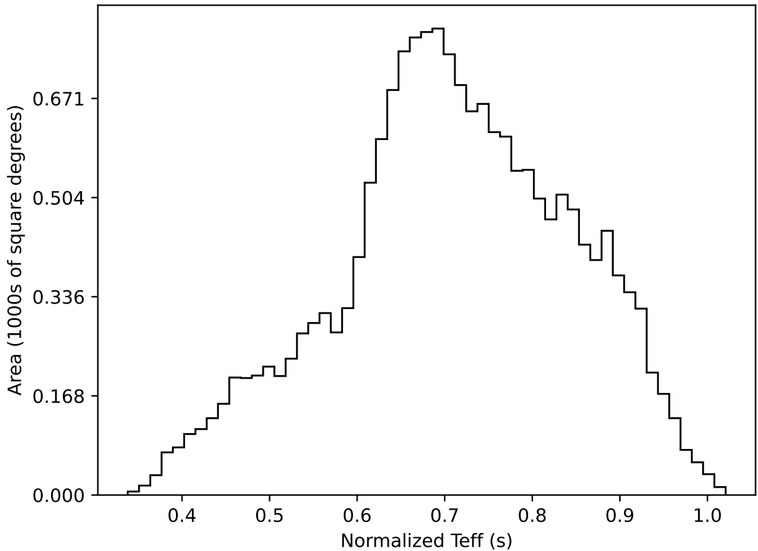
ddf_acor_sf20_lsf0_lsr0_v3.4_10yrs WFD all bands: Normalized Teff
