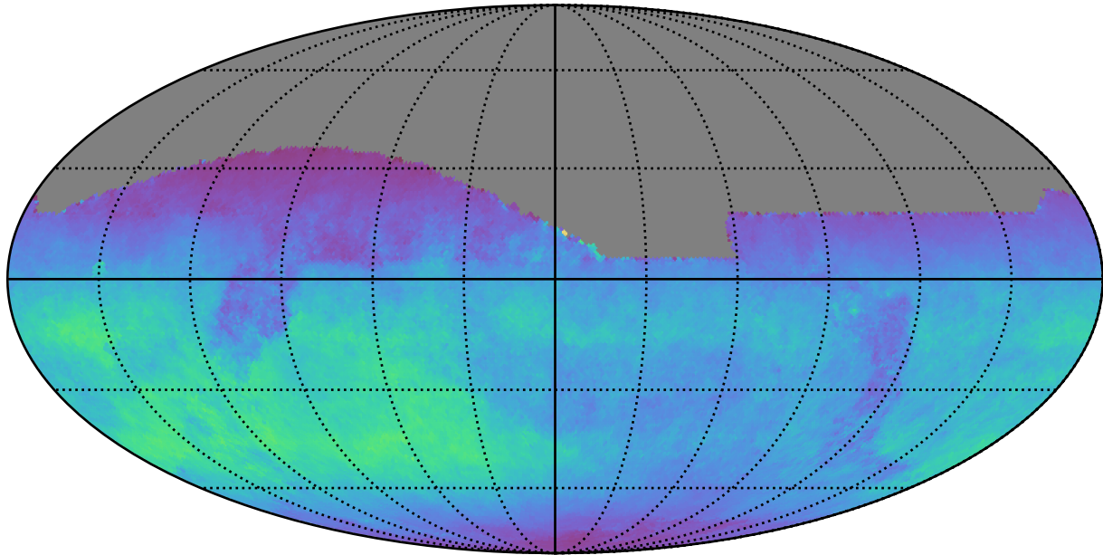
ddf_acor_sf20_lsf0_lsr0_v3.4_10yrs All sky z band: Normalized Teff
