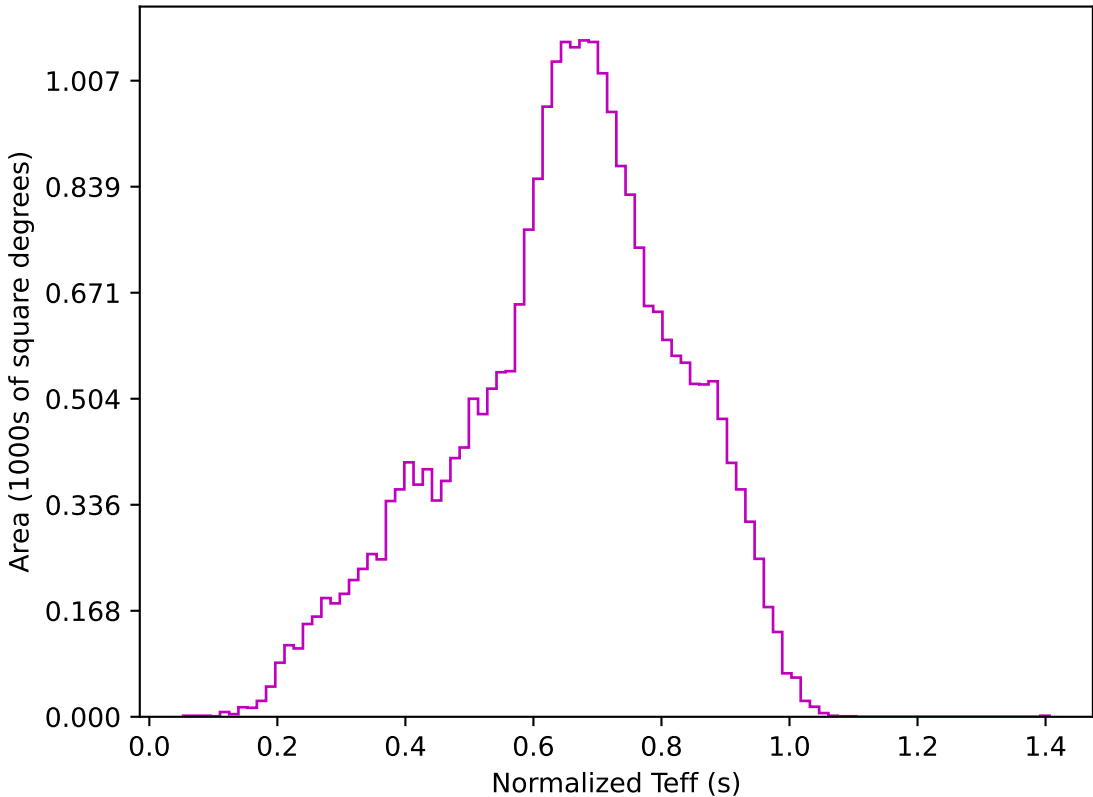
ddf_acor_sf20_lsf0_lsr0_v3.4_10yrs All sky z band: Normalized Teff
