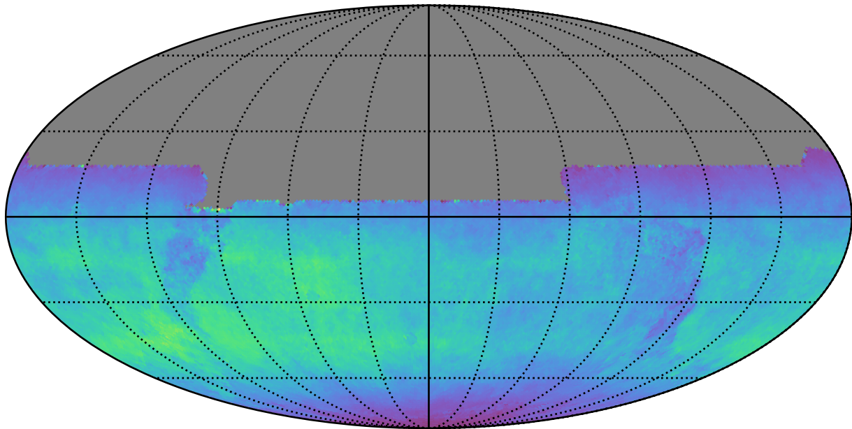
ddf_acor_sf20_lsf0_lsr0_v3.4_10yrs All sky y band: Normalized Teff
