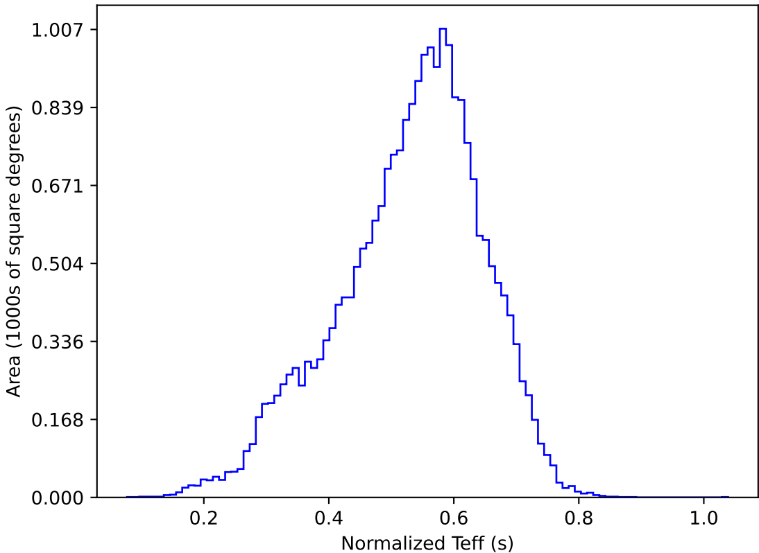
ddf_acor_sf20_lsf0_lsr0_v3.4_10yrs All sky y band: Normalized Teff
