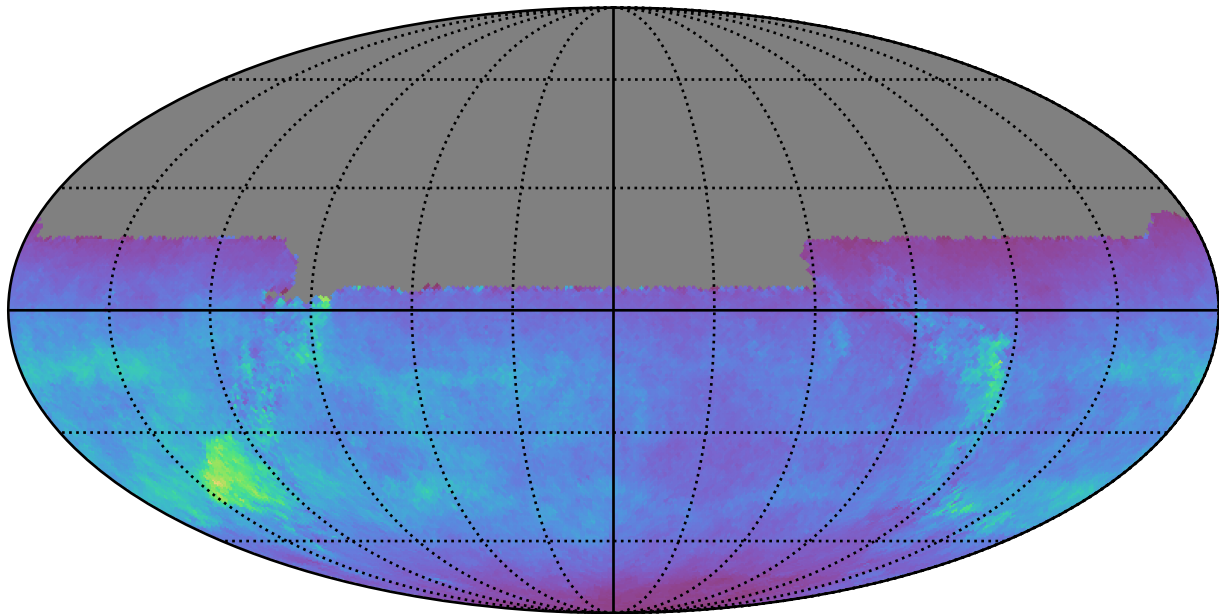
ddf_acor_sf20_lsf0_lsr0_v3.4_10yrs All sky u band: Normalized Teff
