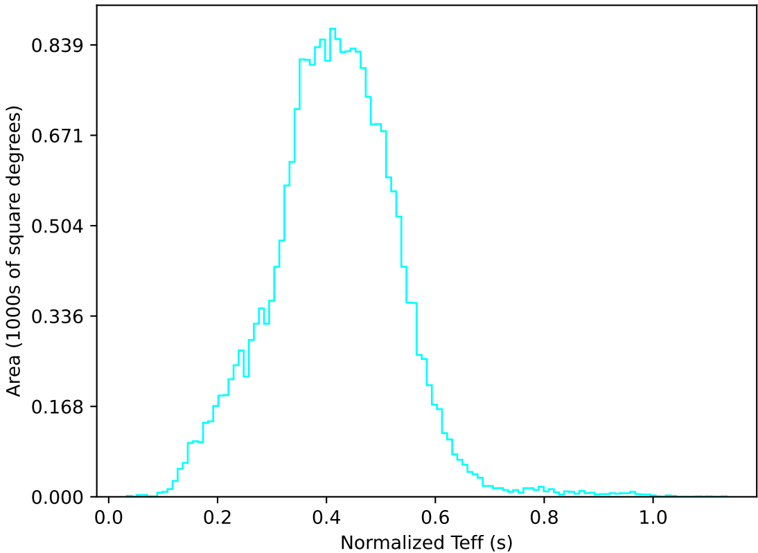
ddf_acor_sf20_lsf0_lsr0_v3.4_10yrs All sky u band: Normalized Teff
