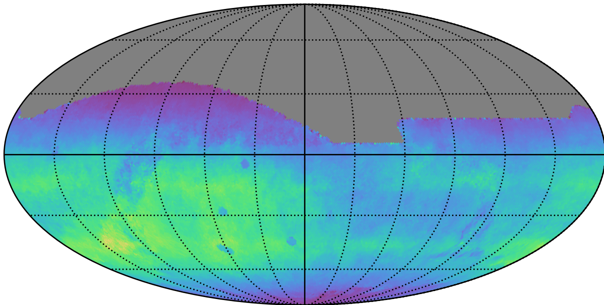
ddf_acor_sf20_lsf0_lsr0_v3.4_10yrs All sky r band: Normalized Teff
