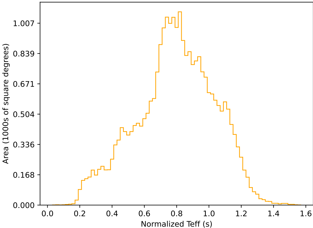
ddf_acor_sf20_lsf0_lsr0_v3.4_10yrs All sky r band: Normalized Teff
