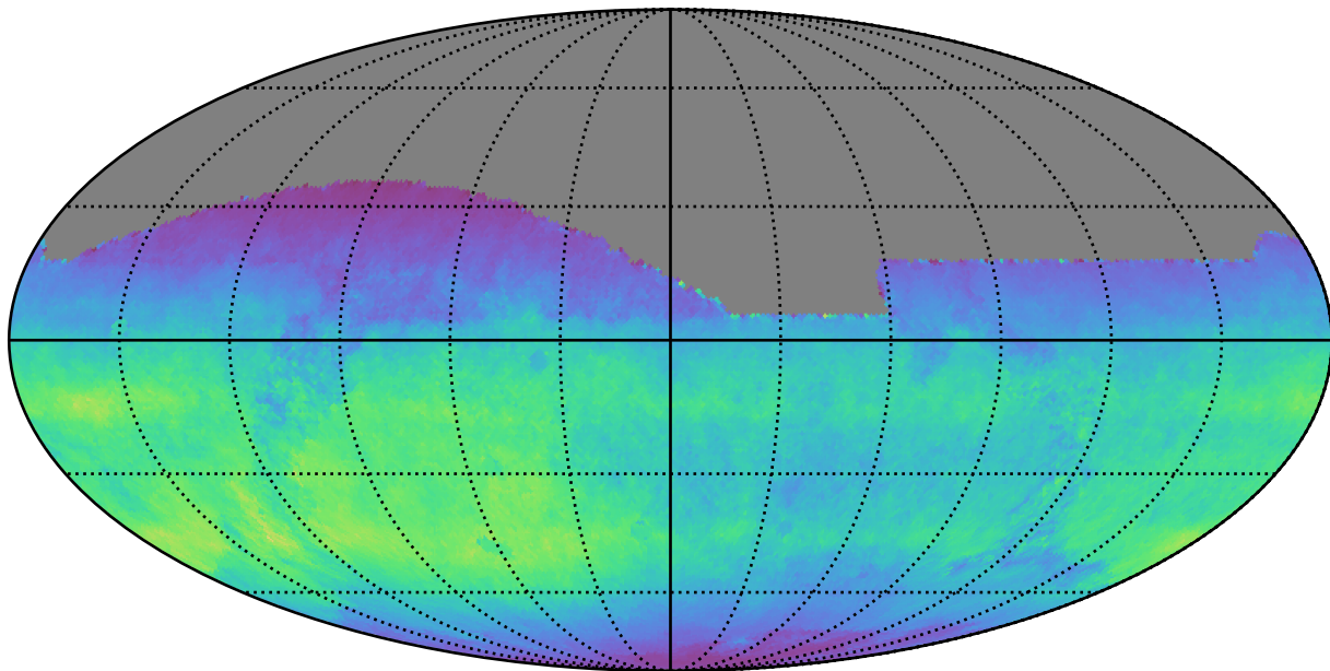
ddf_acor_sf20_lsf0_lsr0_v3.4_10yrs All sky i band: Normalized Teff
