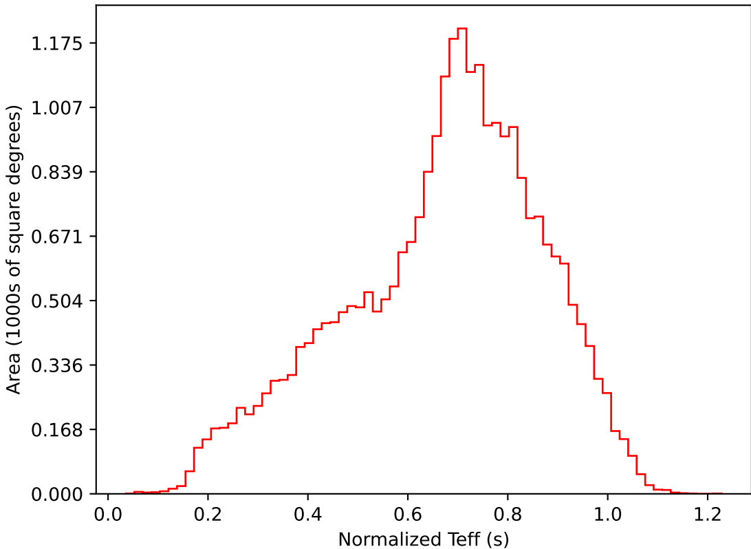
ddf_acor_sf20_lsf0_lsr0_v3.4_10yrs All sky i band: Normalized Teff
