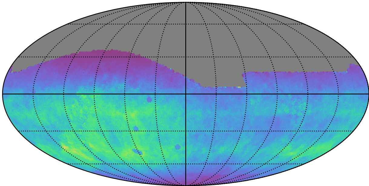
ddf_acor_sf20_lsf0_lsr0_v3.4_10yrs All sky g band: Normalized Teff
