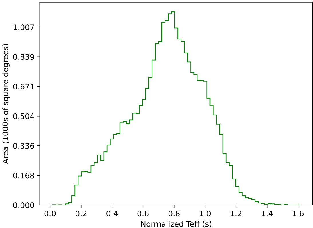
ddf_acor_sf20_lsf0_lsr0_v3.4_10yrs All sky g band: Normalized Teff
