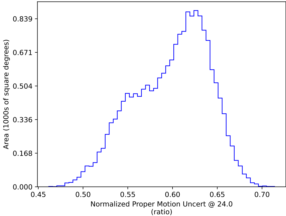
ddf_acor_sf20_lsf0_lsr0_v3.4_10yrs WFD: Normalized Proper Motion Uncert @ 24.0
